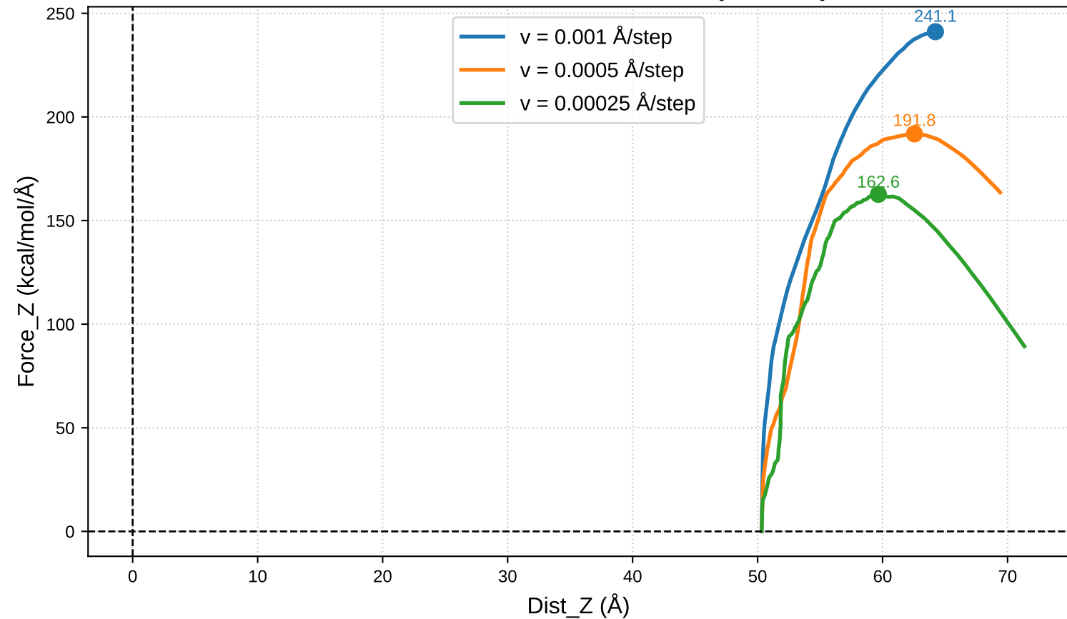
SMD Force-Extension Curves (R1-max)
